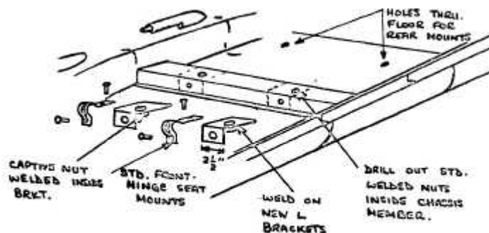
Reinforced seat mounting arrangement
